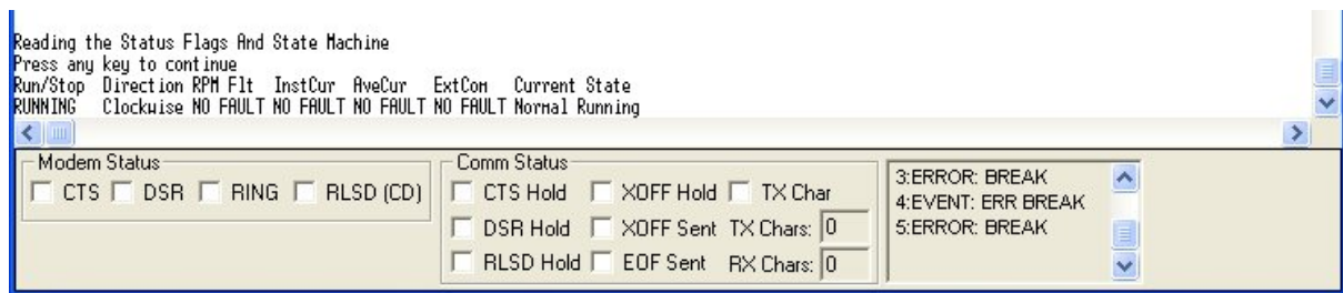
Fig.7.5 Reading the status information from the slave
