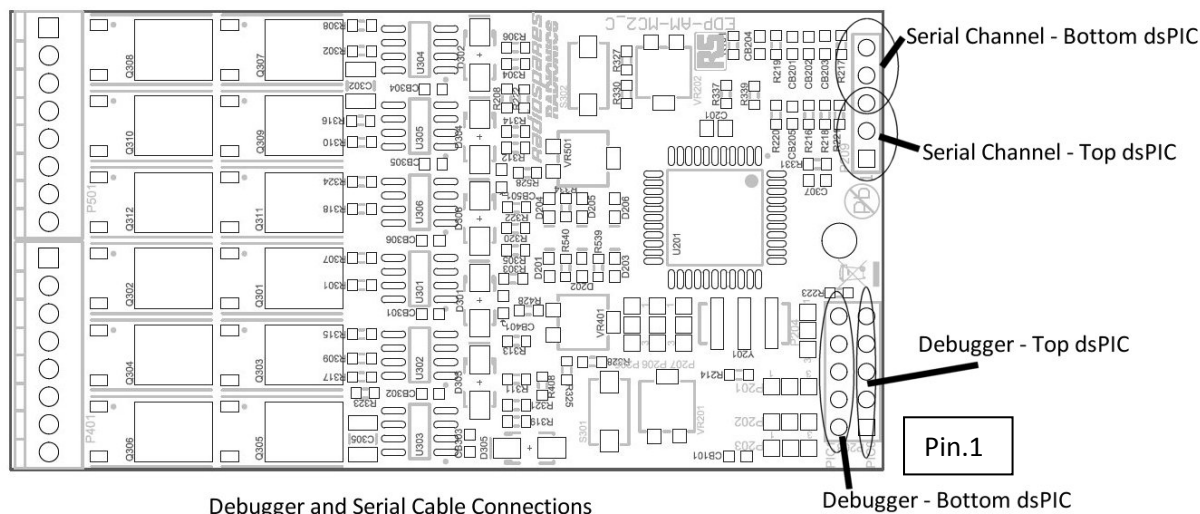
Fig.5.1 Debugger and serial cable connections
