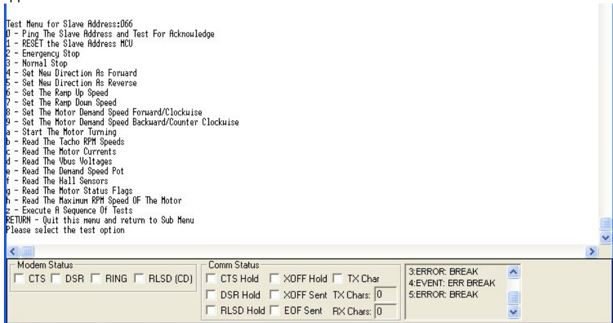
Fig.7.4 I2C command menu
