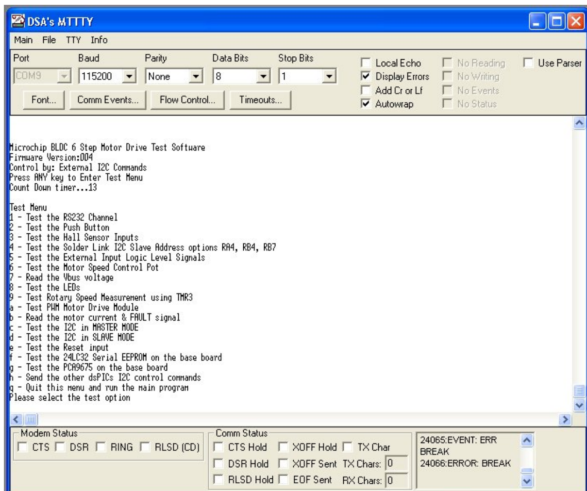
Fig.7.1 Terminal screen shot of menu options
