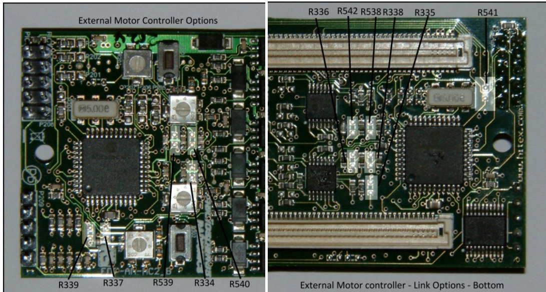
Fig.4.7 External motor control link options
