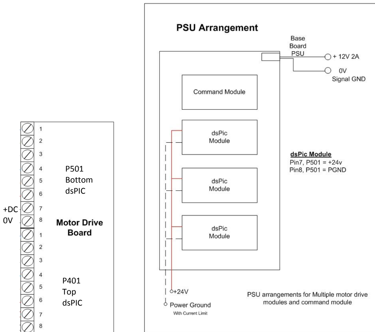
Fig.5.0 PSU connections for BLDC modules
