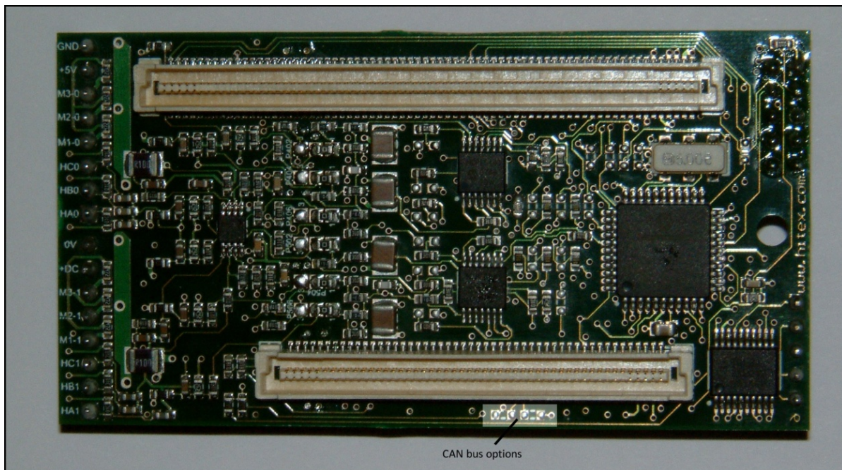
Fig.4.3 Link options for the CAN bus
