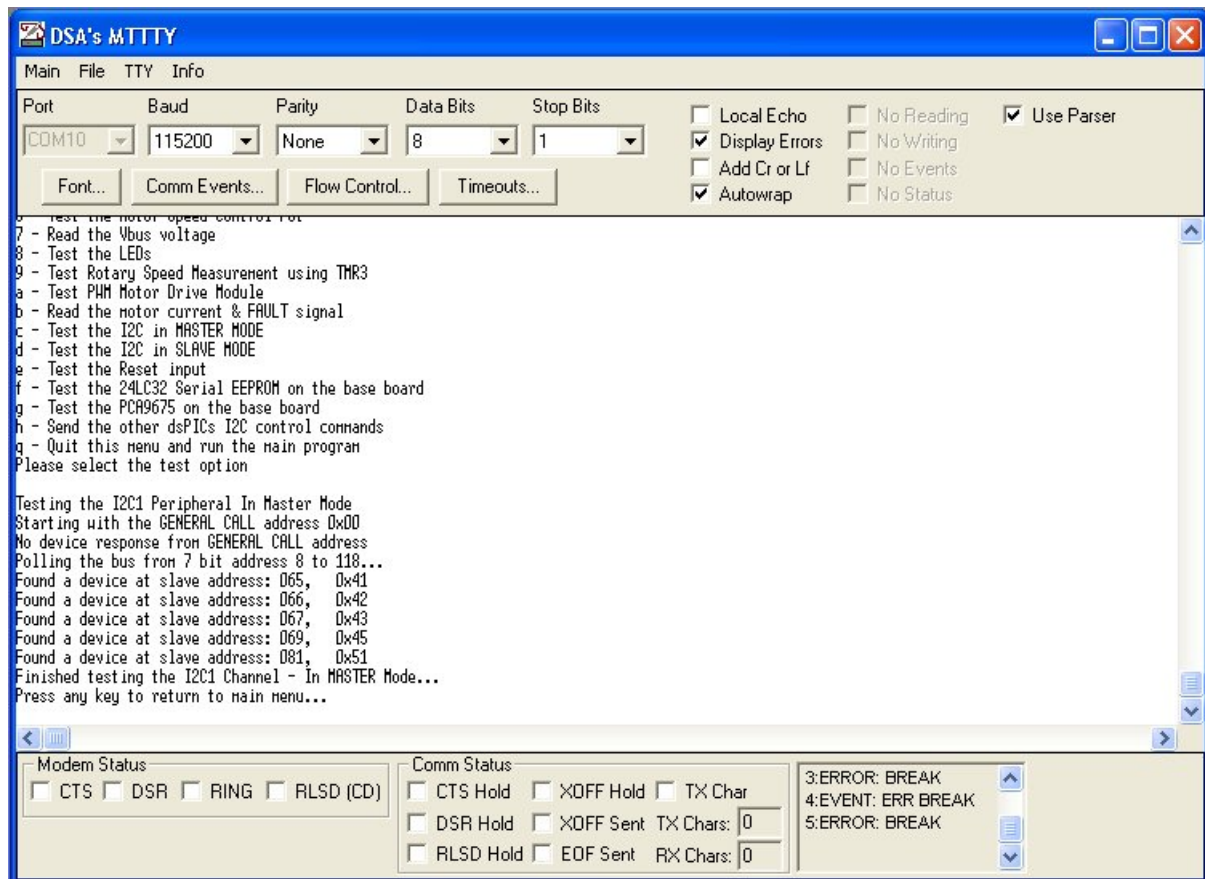
Fig.7.2 I2C master mode menu output
