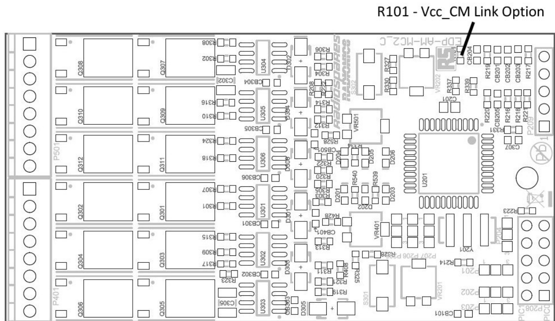
Fig.4.1 Vcc_CM Link option for PCB revision C or later
