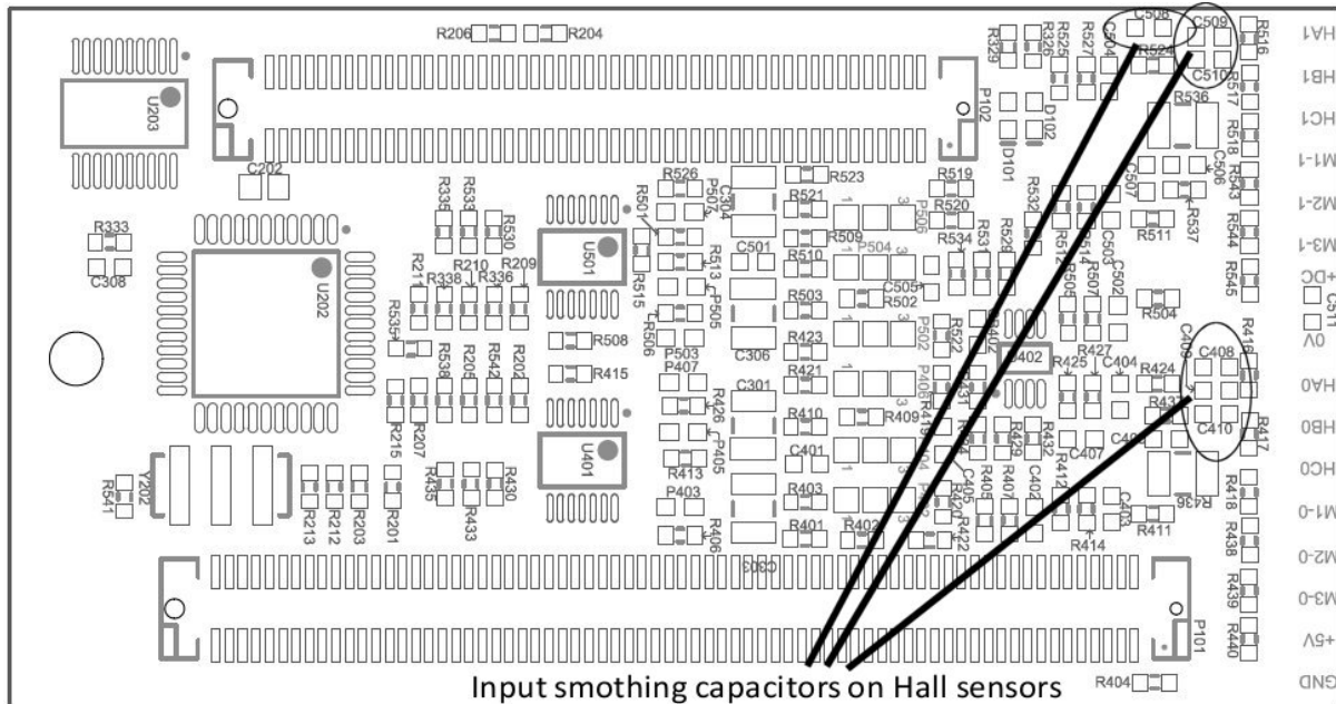
Fig.4.8 Hall sensor capacitors which need to be removed for quad encoder operation
