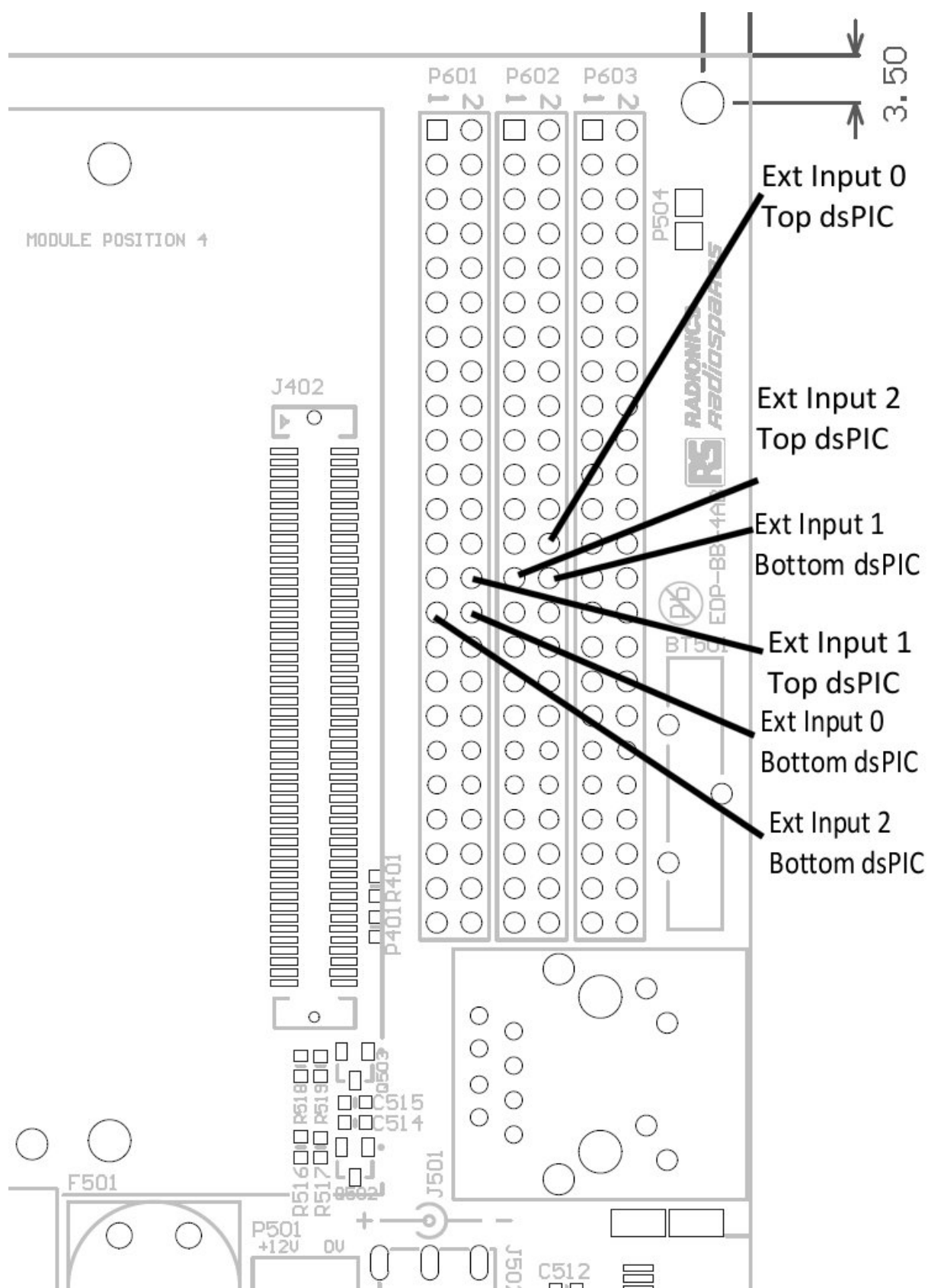
Fig.5.4 Wiring diagram for home sensors
