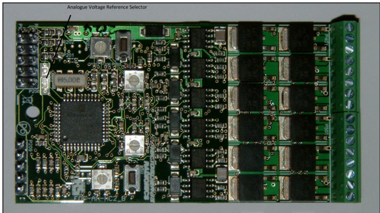
Fig.4.4 Analogue voltage reference selector link option
