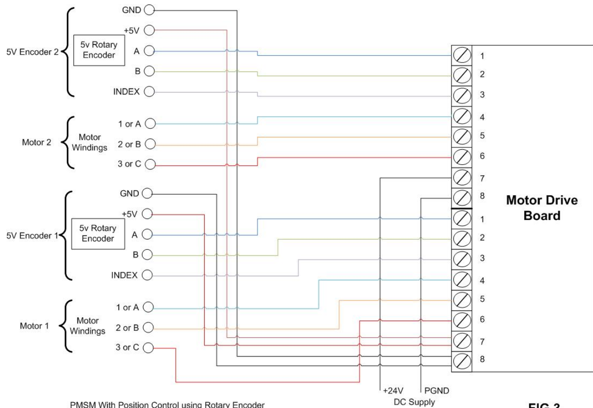
Fig.5.3 Motor connections for PMSM with position control using rotary encoder
